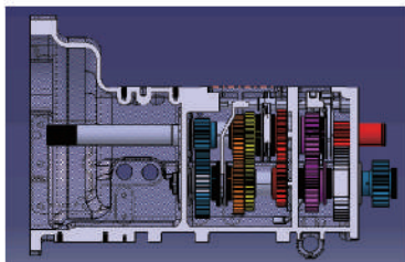
12F+12R shift, optional synchronizer for gear shift. New optimized design for gearbox gear and bearing with the stronger bearing capacity and reasonable speed range.
